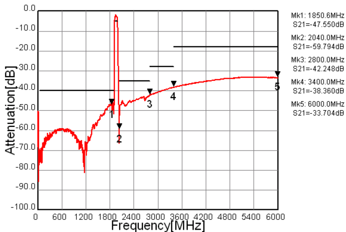
Fig.3 Wide-band Characteristics
