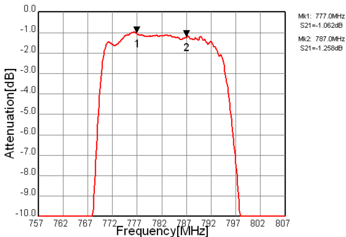
Fig.2 In-band Characteristic
