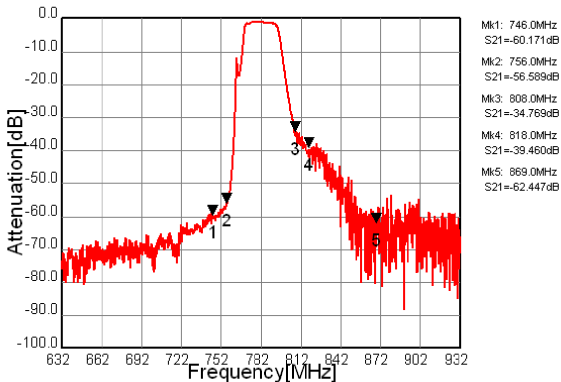
Fig.1 Pass-band Characteristic
