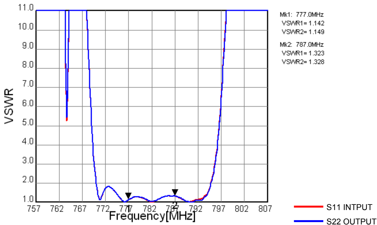
Fig.3 VSWR
