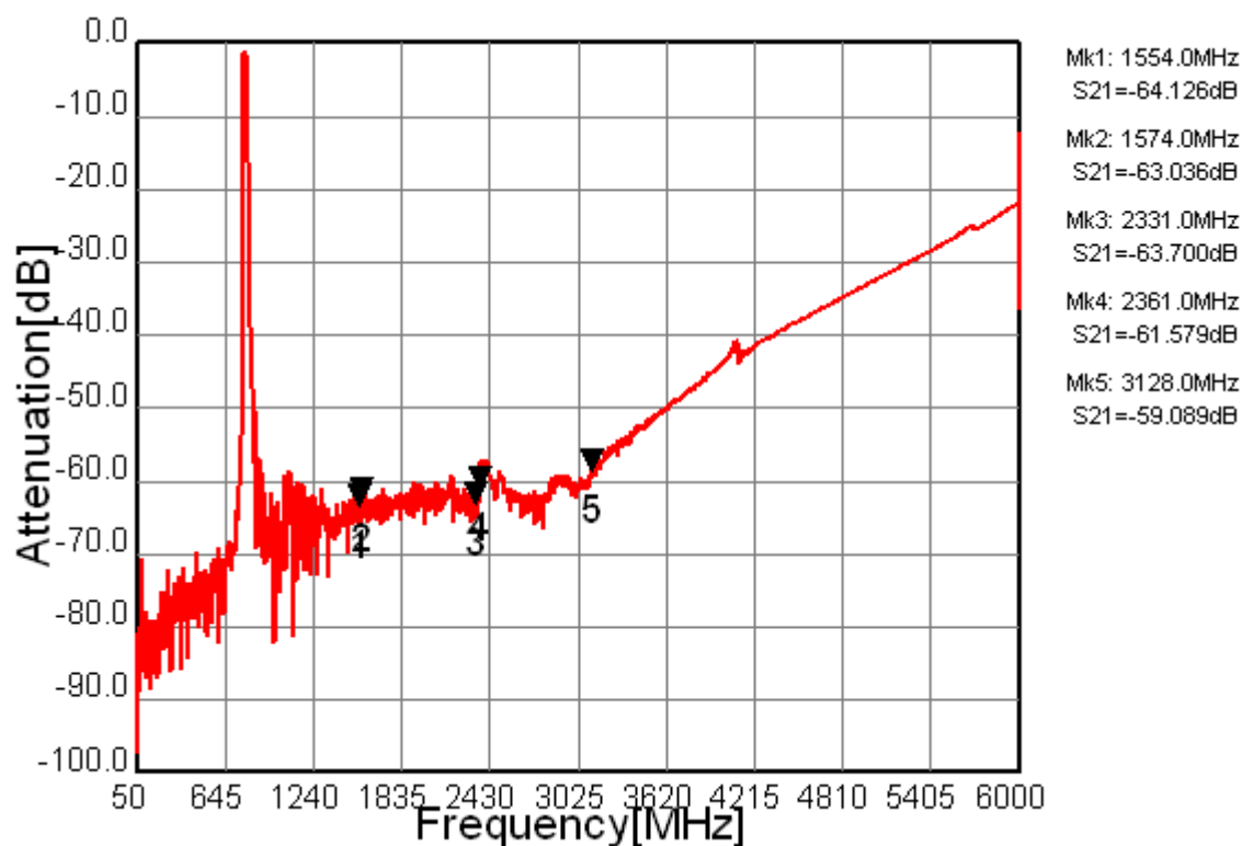
Fig.4 Wide-band Characteristic
