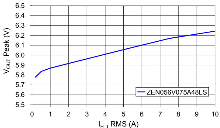
V_{OUT} Peak vs. I_{FLT} RMS ( I_{OUT}=0 )
