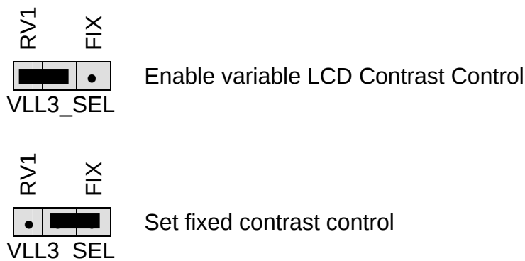
Figure 9: VLL3_SEL Option Header
