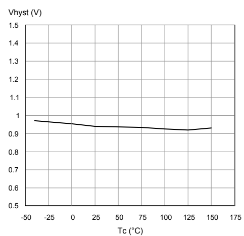
Figure 11. Input hysteresis voltage
