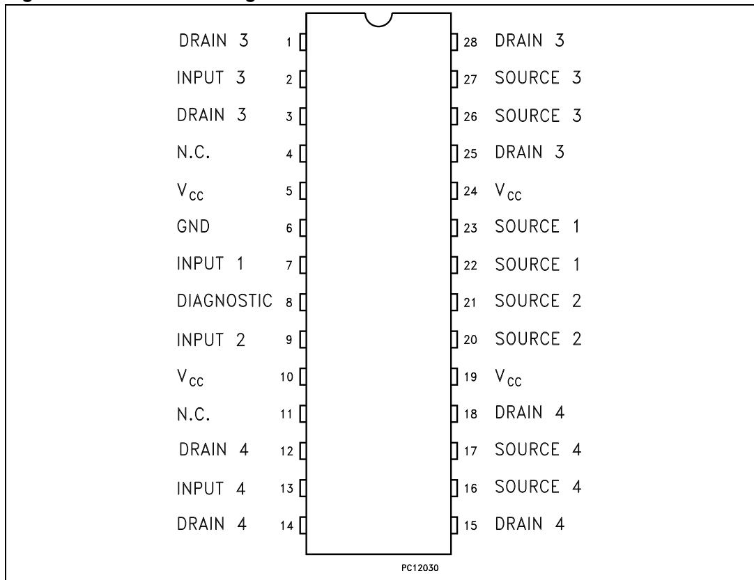
Figure 2. Connection diagram
