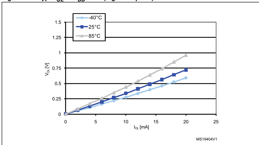
Figure 23. Typ. V_{OL} @ V_{DD} = 5 V (high sink ports)
