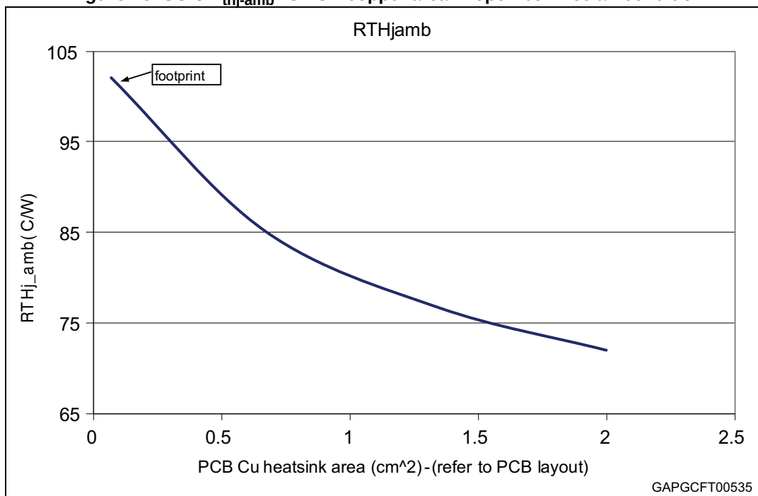
Figure 15. SO-8 R_{thj-amb} vs PCB copper area in open box free air condition
