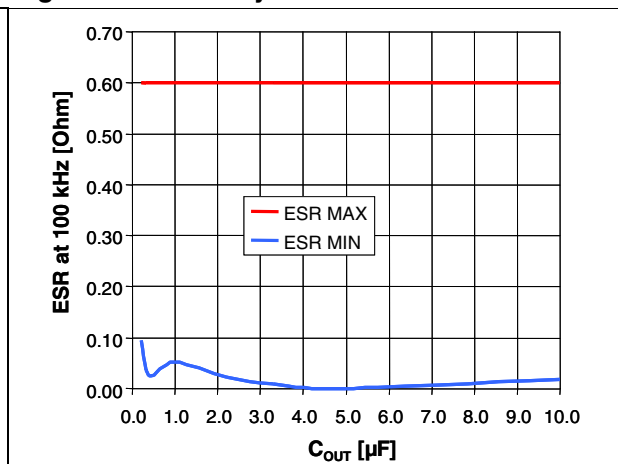
Figure 15. Stability area
