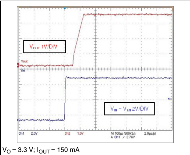
Figure 23. Startup transient
