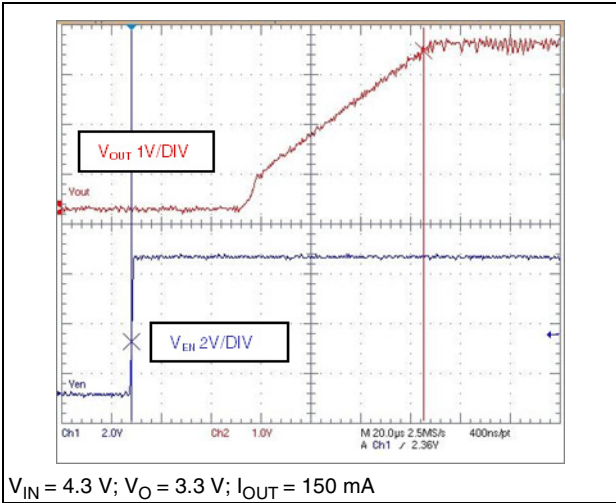
Figure 22. Turn-on time at I_{OUT}=150\text{ mA} , V_{OUT}=3.3\text{ V}
