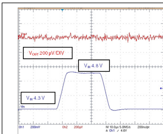
Figure 18. Line transient at I_{OUT} = 150 mA
