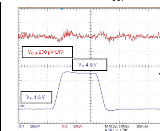
Figure 17. Line transient at I_{OUT} = 1 mA
