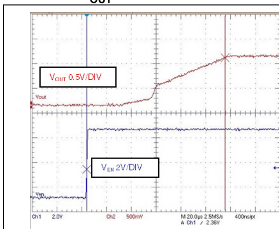
Figure 20. Turn-on time at I_{OUT} = 150 mA, V_{OUT} = 1 V
