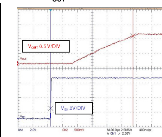
Figure 19. Turn-on time at I_{OUT} = 1 mA; V_{OUT} = 1 V
