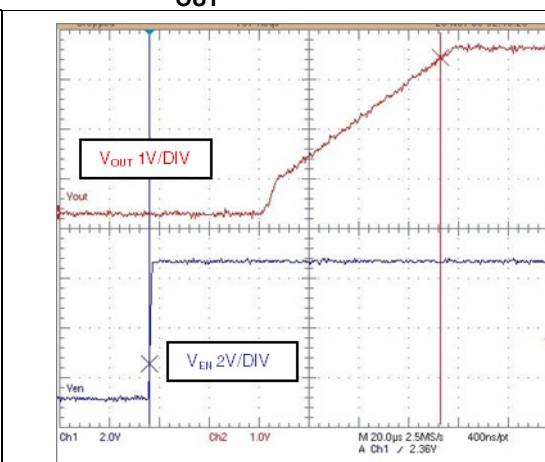
Figure 21. Turn-on time at I_{OUT} = 1 mA; V_{OUT} = 3.3 V
