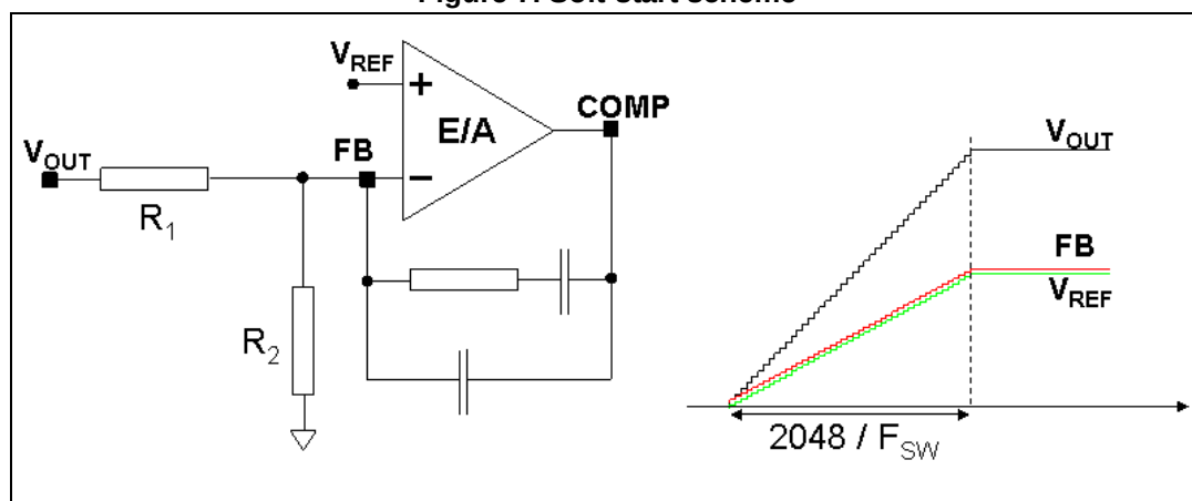
Figure 7. Soft-start scheme
