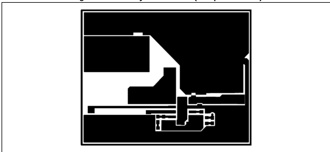
Figure 19. PCB layout: A7986A (component side)
