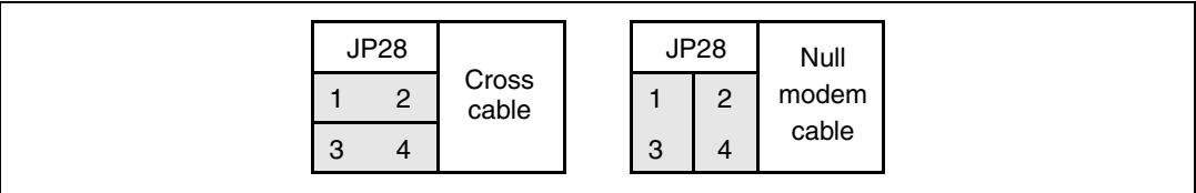
Figure 4. Primary serial cable setting (J34)
