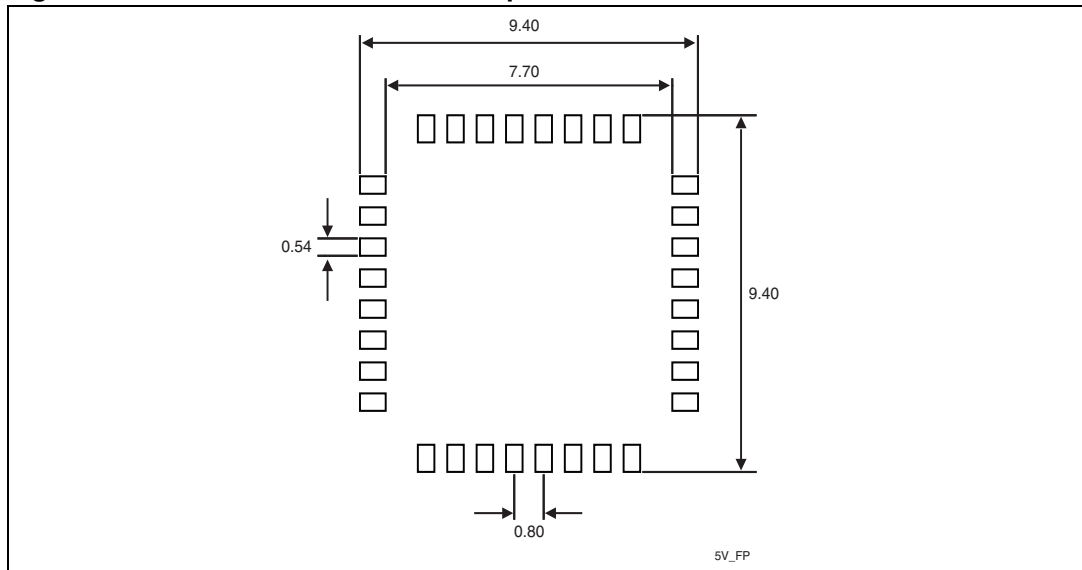
Figure 6. LQFP48 recommended footprint
