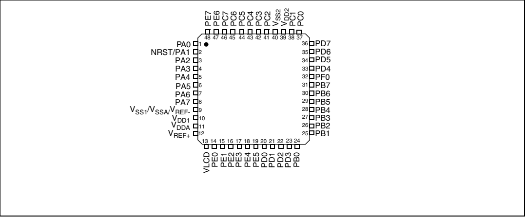
Figure 3. STM8L052C6 48-pin LQFP48 package pinout (with LCD)
