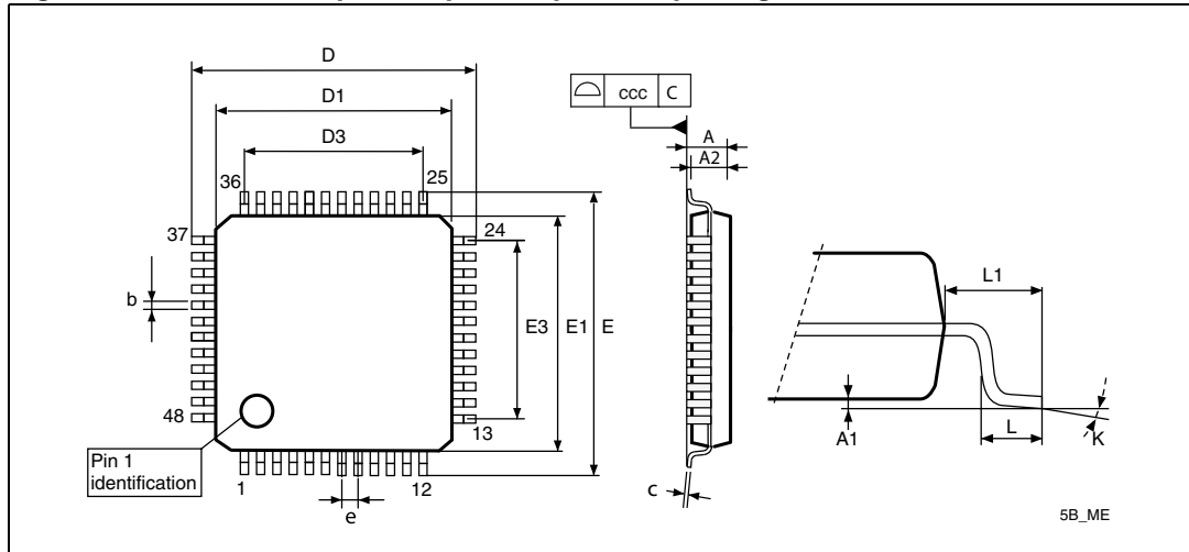
Figure 5. LQFP48 48-pin low profile quad flat package outline
