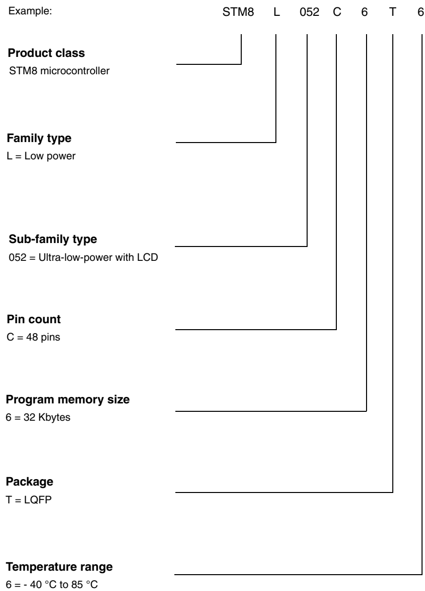
Figure 7. Medium density value line STM8L05xxx ordering information scheme
