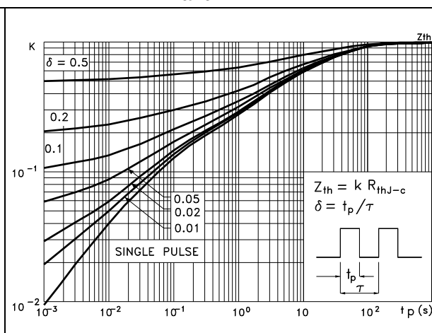
Figure 3. Thermal impedance DPAK, TO-220 and IPAK
