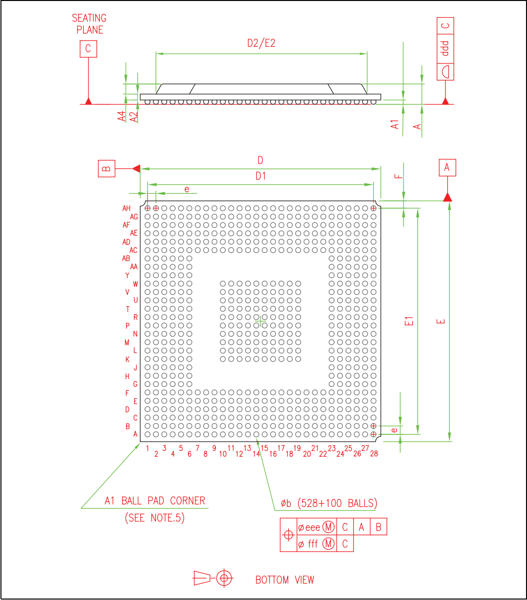
Figure 52. PGBA package - bottom view
