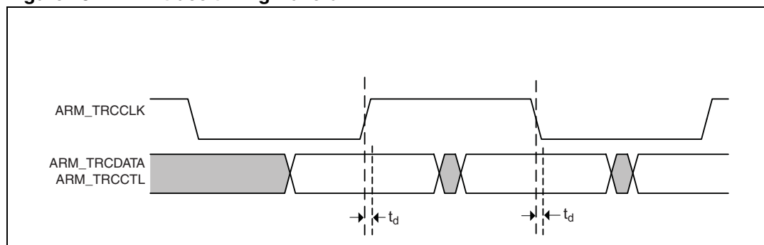
Figure 18. ARM trace timing waveform
