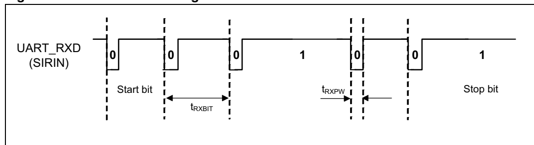
Figure 49. IrDA receive timing waveform
