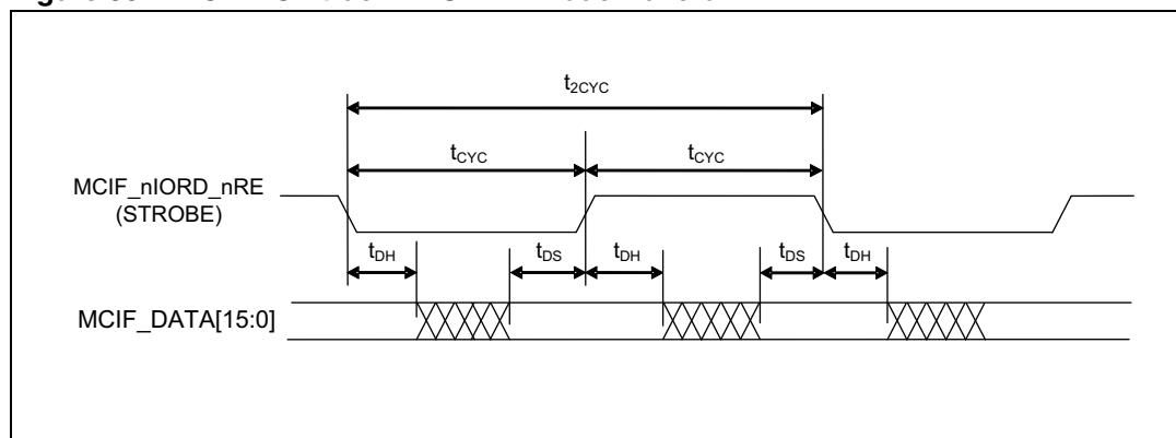
Figure 36. MCIF - CF true IDE UDMA mode waveform
