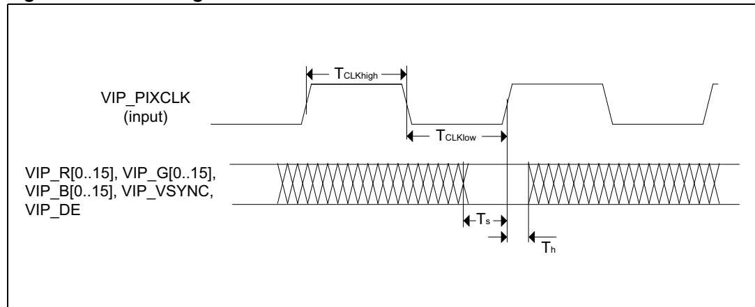
Figure 50. VIP timing waveform
