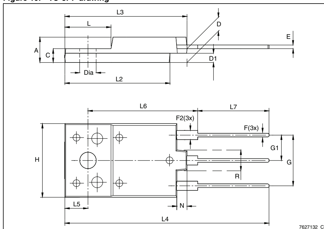
Figure 19. TO-3PF drawing
