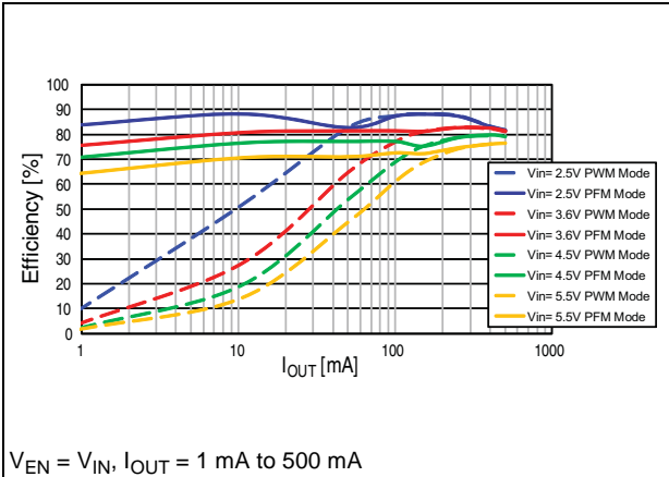
Figure 3. Efficiency vs. output current ( V_{OUT} = 1.82\text{ V} )
