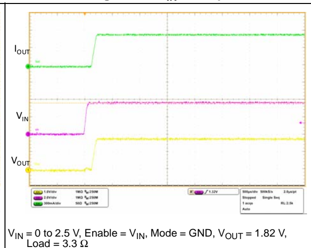
Figure 20. V_{IN} startup
