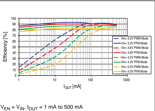
Figure 4. Efficiency vs. output current ( V_{OUT} = 2.8\text{ V} )
