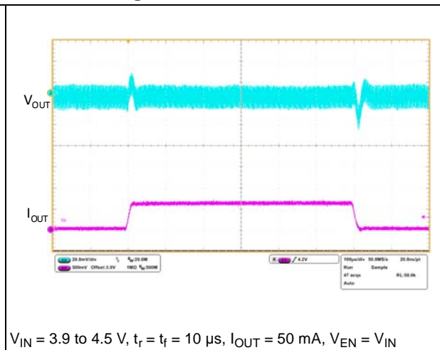
Figure 16. Line transient
