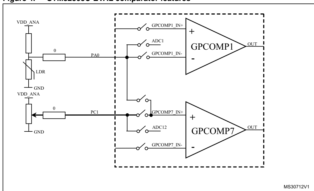
Figure 4. STM32303C-EVAL comparator features
