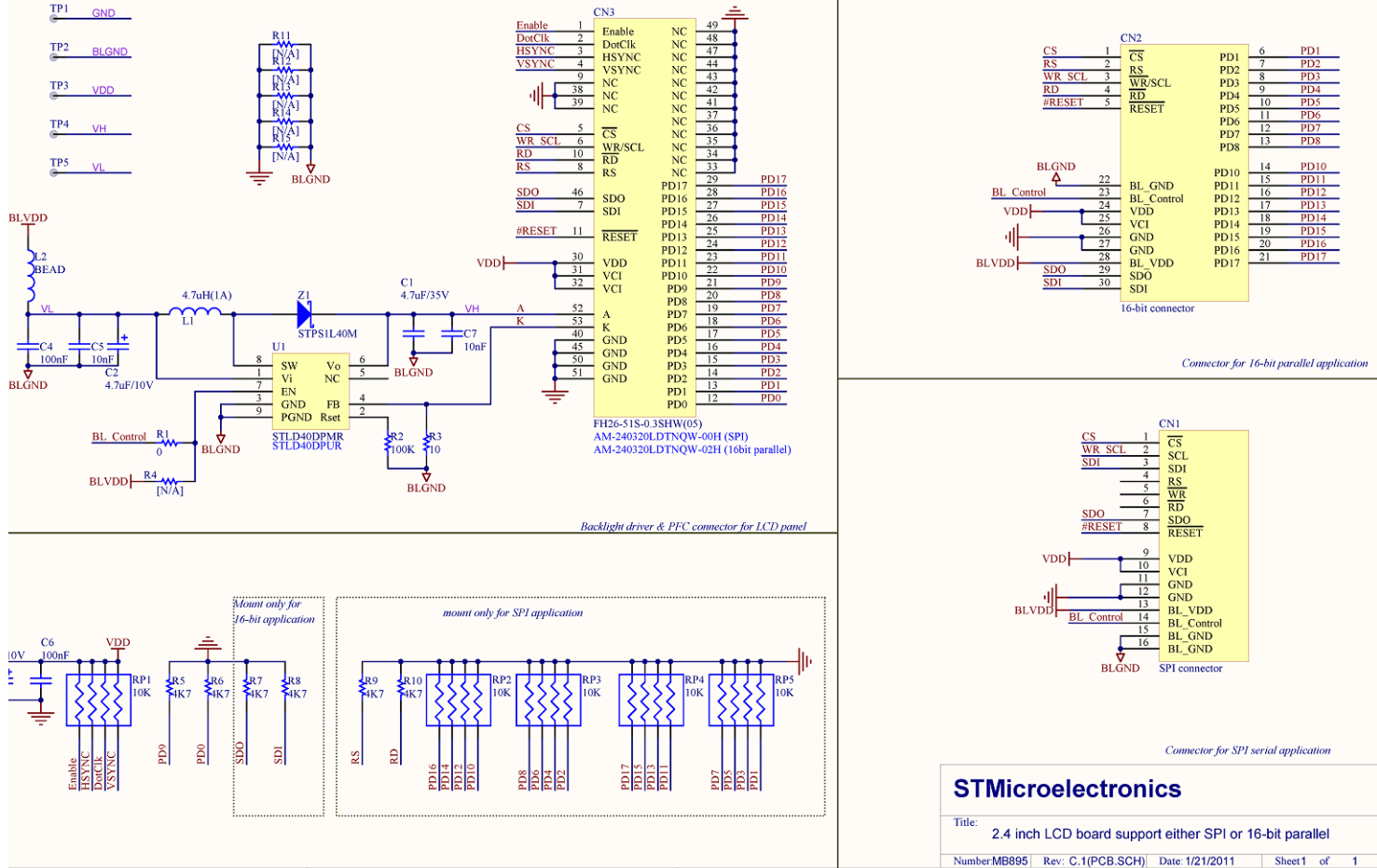
Figure 31. Color LCD daughter board (MB895)
