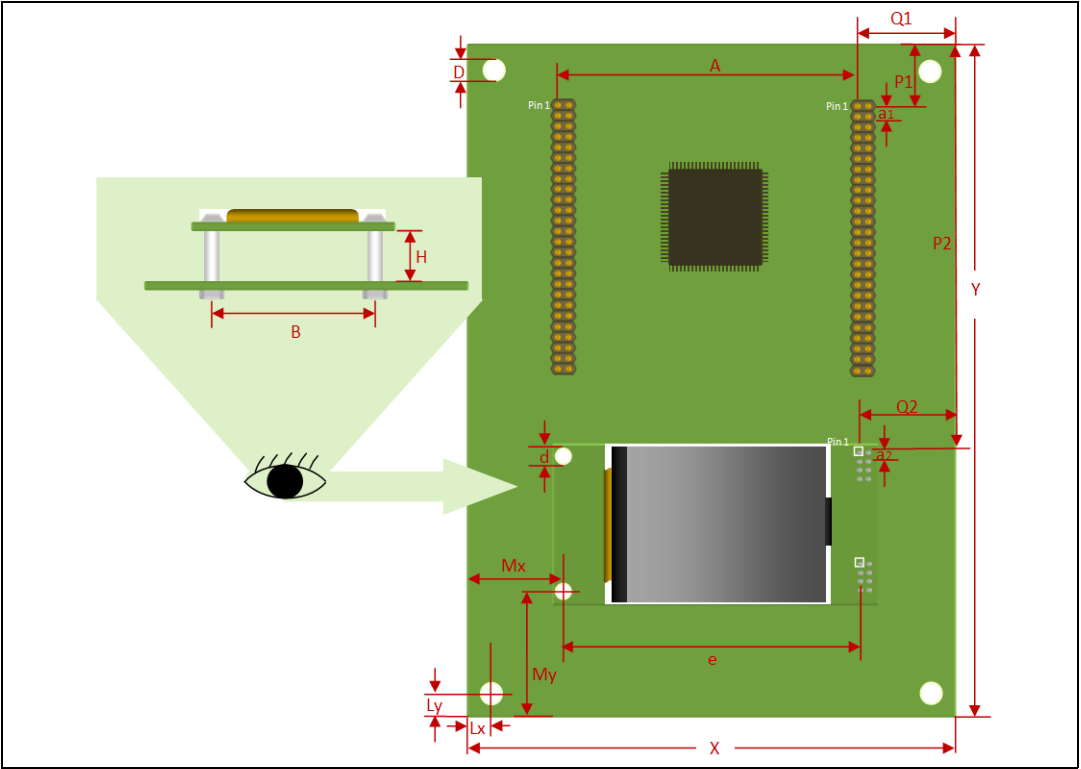
Figure 32. Mechanical dimensions
