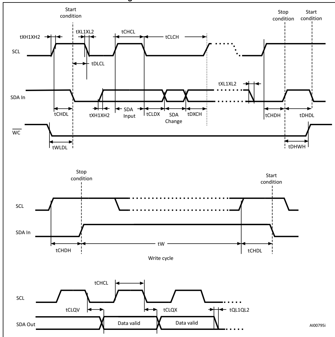
Figure 12. AC waveforms
