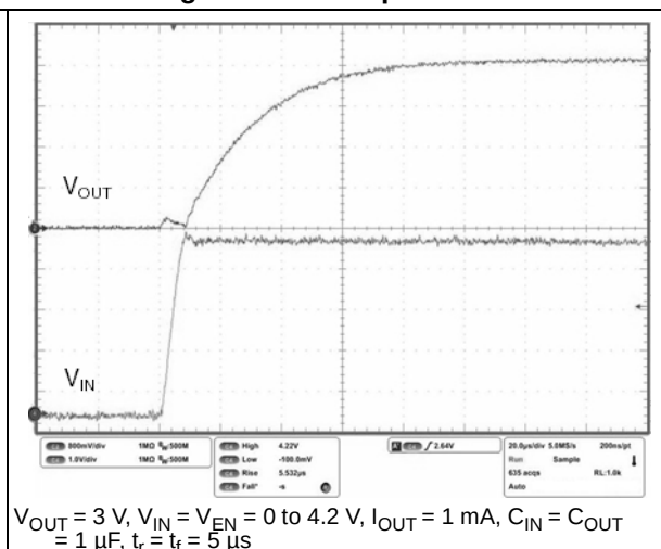
Figure 30. Startup transient
