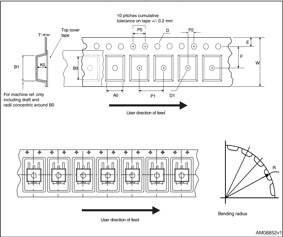
Figure 24. Tape drawing
