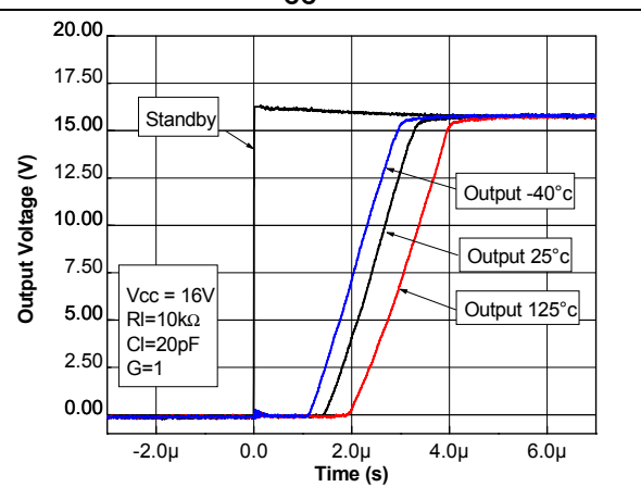
Figure 37. Startup time after standby released for V_{CC} = 16\text{ V}
