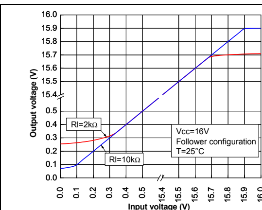
Figure 13. Output rail linearity
