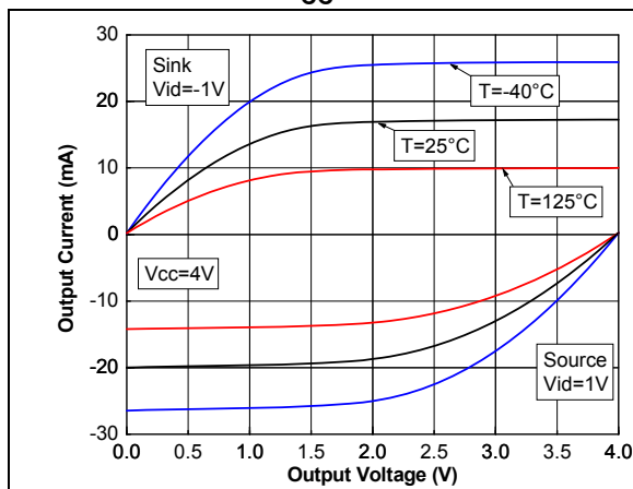
Figure 10. Output current vs. output voltage at V_{CC} = 4\text{ V}
