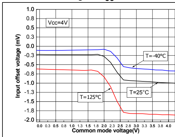
Figure 8. Input offset voltage vs. common mode voltage at V_{CC} = 4\text{ V}
