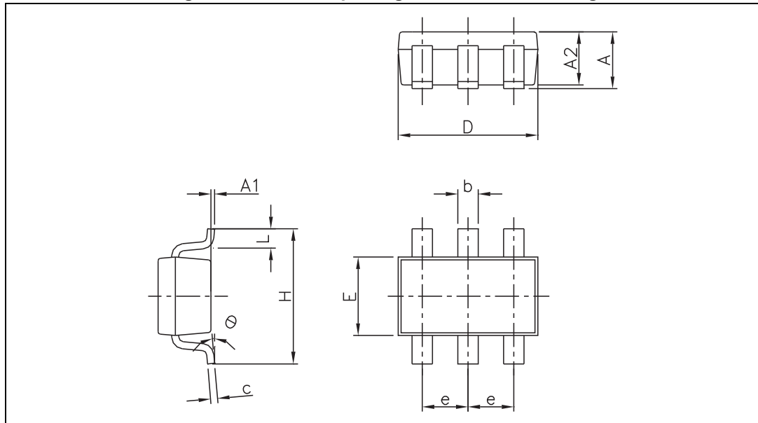
Figure 44. SOT23-6 package mechanical drawing
