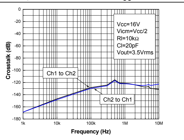
Figure 35. Crosstalk vs. frequency between operators on TSX922 at V_{CC} = 16\text{ V}
