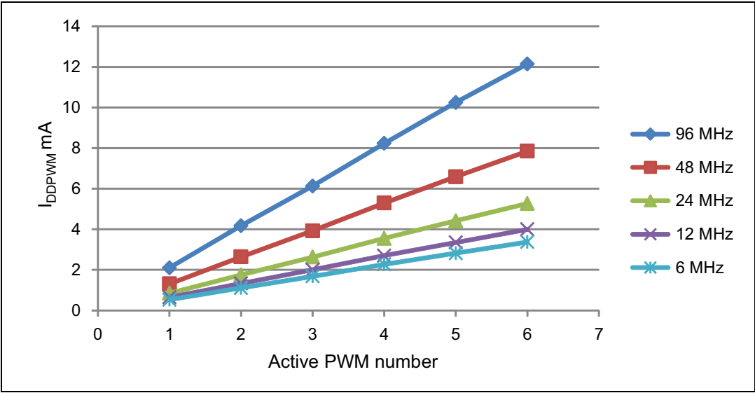
Figure 13. PWM current consumption with f_{\text{SMED}}=\text{PLL} f_{\text{PWM}}=0.5 MHz at V_{\text{DD}}/V_{\text{DDA}}=3.3\text{V}
