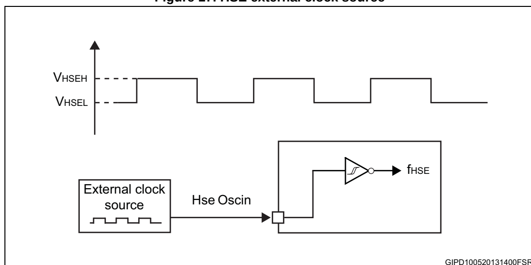
Figure 17. HSE external clock source
