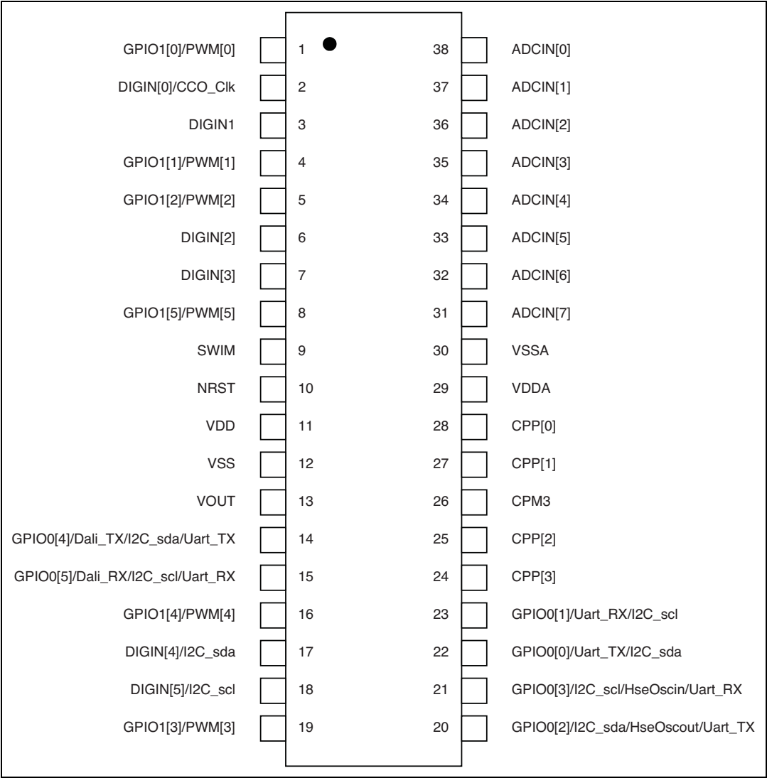
Figure 6. TSSOP38 pinout
