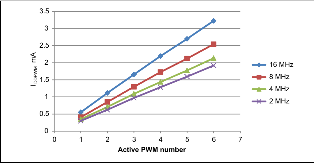
Figure 14. PWM current consumption with f_{\text{SMED}}=\text{PLL} f_{\text{PWM}}=0.5 MHz at V_{\text{DD}}/V_{\text{DDA}}=5\text{V}
