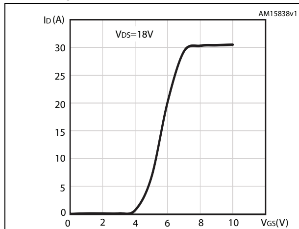
Figure 6. Transfer characteristics
