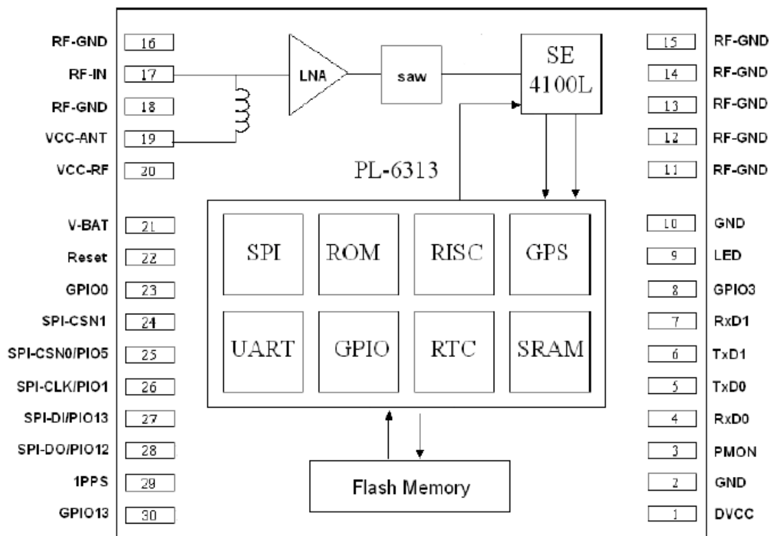
Figure 3-1 Block Diagram
