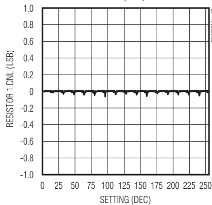
RESISTOR 1 DNL (LSB) vs. SETTING
