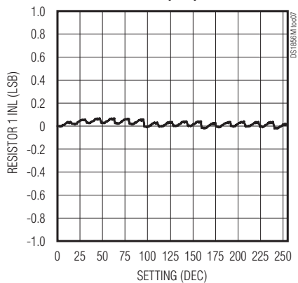
RESISTOR 1 INL (LSB) vs. SETTING
