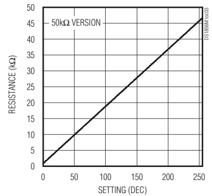
RESISTANCE vs. SETTING
