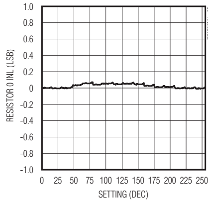
RESISTOR 0 INL (LSB) vs. SETTING
