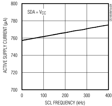
ACTIVE SUPPLY CURRENT vs. SCL FREQUENCY
