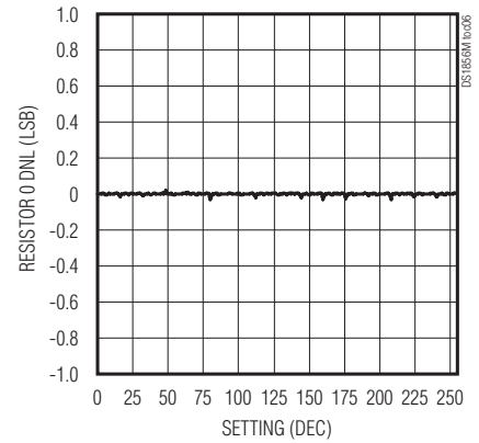
RESISTOR 0 DNL (LSB) vs. SETTING
