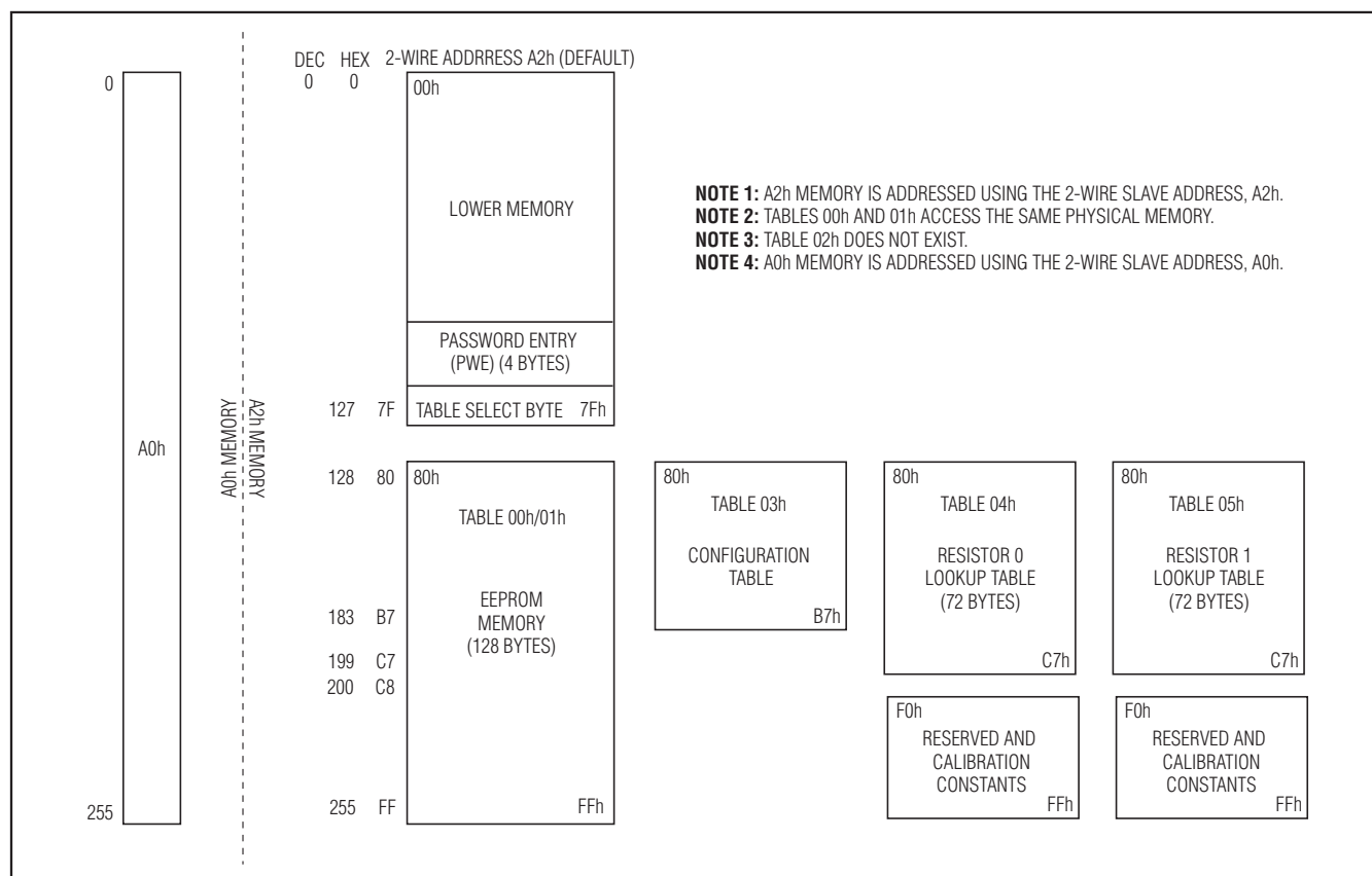
Figure 2. Memory Organization
