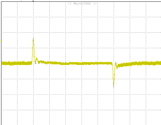
Figure 21: Transient response to dynamic load change at 2.5\text{A}/\mu\text{S} from 50%~ 100%~50% of I_o , max at 12\text{V}_{in} , 3.3\text{V}_{out} ( C_{out} = 1\mu\text{F} ceramic, 47\mu\text{F} \times 2 + 10\mu\text{F} ceramic) Yellow : V_{OUT} , 0.2\text{V}/\text{div} , 100\mu\text{S}/\text{div}
