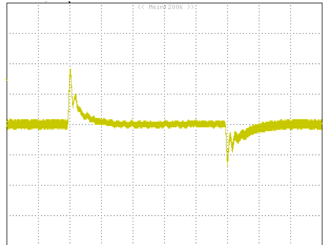
Figure 22: Transient response to dynamic load change at 2.5\text{A}/\mu\text{S} from 50%~ 100%~50% of I_o , max at 12\text{V}_{in} , 5\text{V}_{out} ( C_{out} = 1\mu\text{F} ceramic, 47\mu\text{F} \times 2 + 10\mu\text{F} ceramic) Yellow : V_{OUT} , 0.2\text{V}/\text{div} , 100\mu\text{S}/\text{div}
