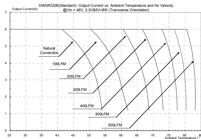
Figure 14: Output current vs. ambient temperature and air velocity @Vin=48V (Transverse Orientation, Pout2 = 8 W (Vout2=3.3V), Pout3 = 0.5 W (Vout3=5V)
