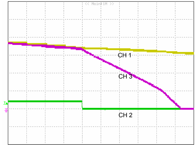
Figure 2: Input voltage turn-off threshold (2mS/div):
