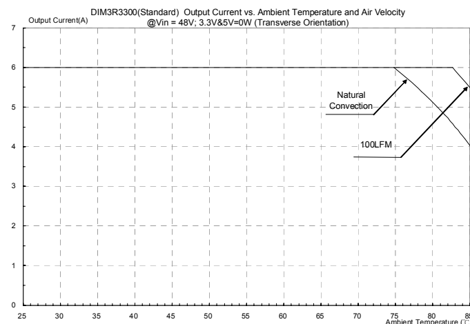
Figure 15: Output current vs. ambient temperature and air velocity @Vin=48V (Transverse Orientation, Pout2 = 0 W (Vout2=3.3V), Pout3 = 0 W (Vout3=5V)
