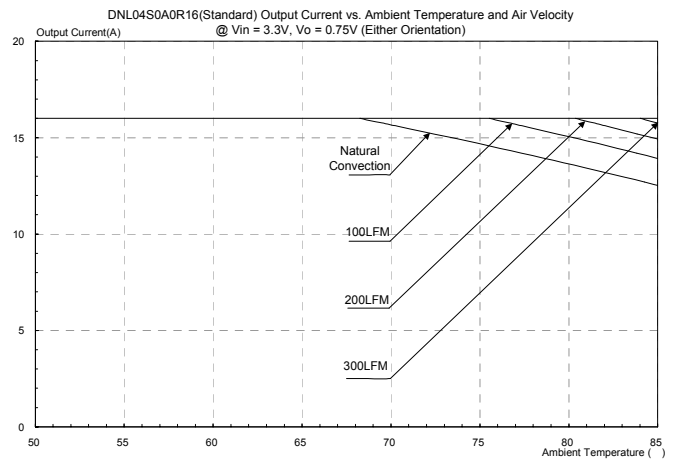
Figure 50: DNL04S0A0R16(Standard) output current vs. ambient temperature and air velocity @Vin=3.3V, Vo=0.75V(Either Orientation).
