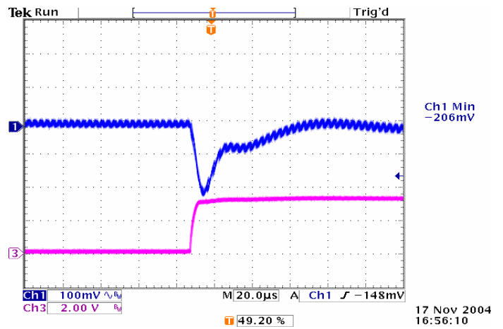
Figure 20: Typical transient response to step load change at 2.5A/\mu S from 50% to 100% of I_o , max at 5Vin, 3.3V out (Cout = ceramic, 10 \mu F tantalum)
