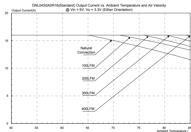
Figure 45: DNL04S0A0R16(Standard) output current vs. ambient temperature and air velocity @ Vin=5V, Vo=3.3V(Either Orientation).
