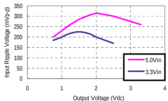
Figure 32: Input voltage ripple for various output models, I_O = 16 A ( C_{IN} = 2 \times 100 µF tantalum // 47 µF ceramic)
