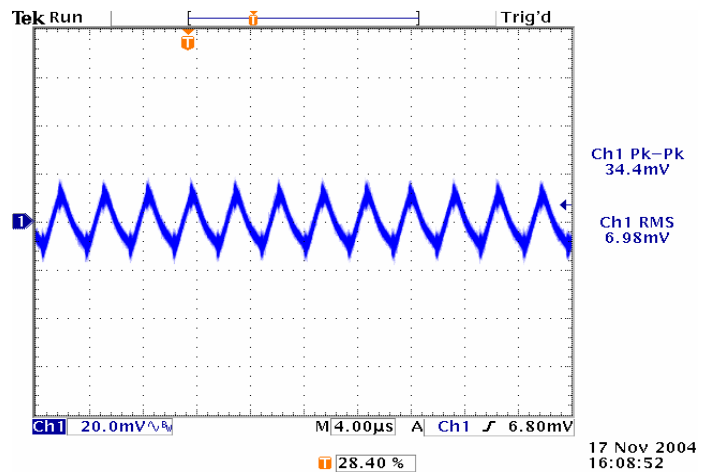
Figure 8: Output ripple & noise at 3.3Vin, 1.8V/16A out
