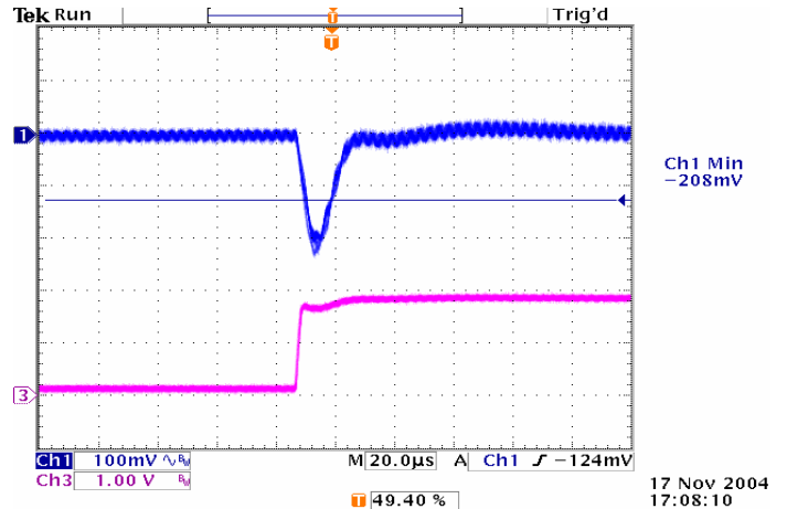
Figure 22: Typical transient response to step load change at 2.5A/\mu S from 50% to 100% of I_o , max at 5Vin, 1.8V out (Cout = ceramic, 10 \mu F tantalum)
