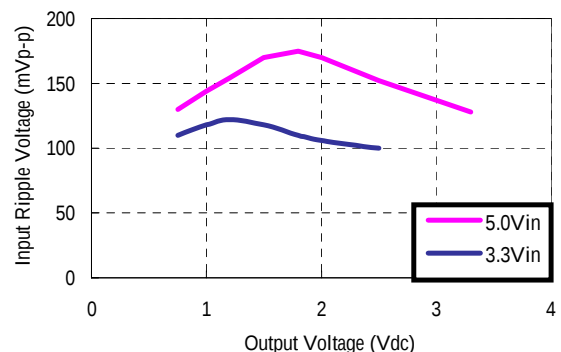
Figure 33: Input voltage ripple for various output models, I_O = 16 A ( C_{IN} = 4 \times 100 µF tantalum // 2 x 47 µF ceramic)
