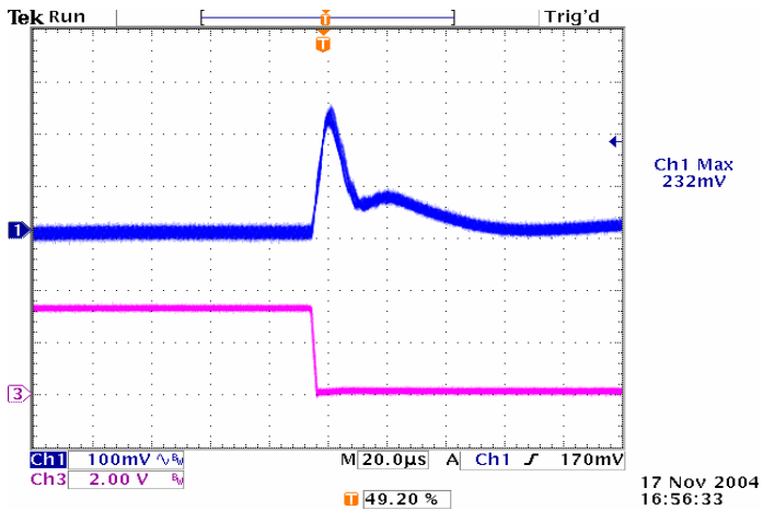
Figure 19: Typical transient response to step load change at 2.5A/\mu S from 100% to 50% of I_o , max at 5Vin, 3.3V out (Cout = ceramic, 10 \mu F tantalum)
