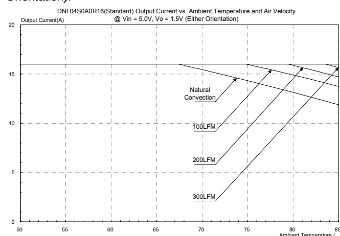
Figure 46: DNL04S0A0R16(Standard) output current vs. ambient temperature and air velocity @ Vin=5V, Vo=1.5V(Either Orientation).
