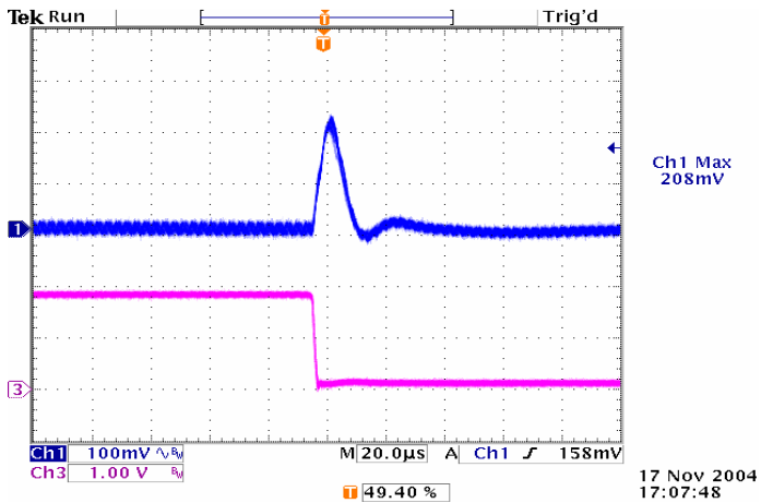
Figure 21: Typical transient response to step load change at 2.5A/\mu S from 100% to 50% of I_o , max at 5Vin, 1.8V out (Cout = ceramic, 10 \mu F tantalum)
