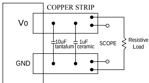
Figure 29: Input reflected-ripple test setup
