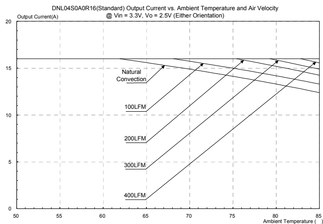
Figure 48: DNL04S0A0R16(Standard) output current vs. ambient temperature and air velocity @Vin=3.3V, Vo=2.5V(Either Orientation).
