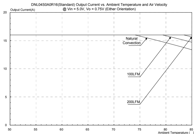
Figure 47: DNL04S0A0R16(Standard) output current vs. ambient temperature and air velocity @Vin=5V, Vo=0.75V(Either Orientation).
