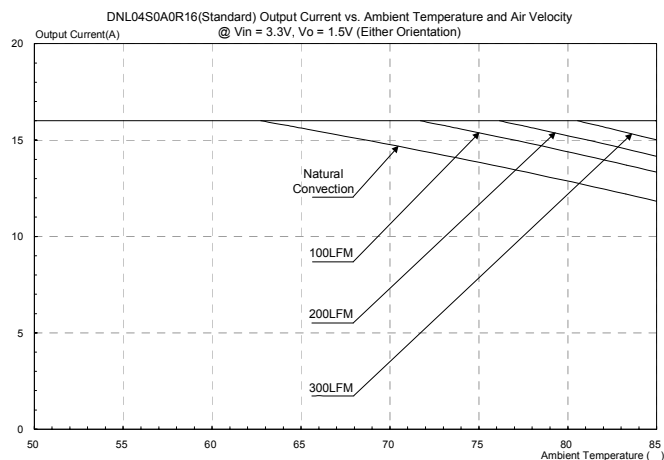
Figure 49: DNL04S0A0R16(Standard) output current vs. ambient temperature and air velocity @Vin=3.3V, Vo=1.5V(Either Orientation).
