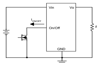
Figure 29: Positive remote On/Off implementation
