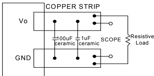
Figure 25: Input reflected-ripple test setup
