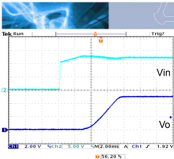
Figure 13: Turn on at 12Vin, with external capacitors ( C_o = 5000 \mu F ), 5.0V/20A out
