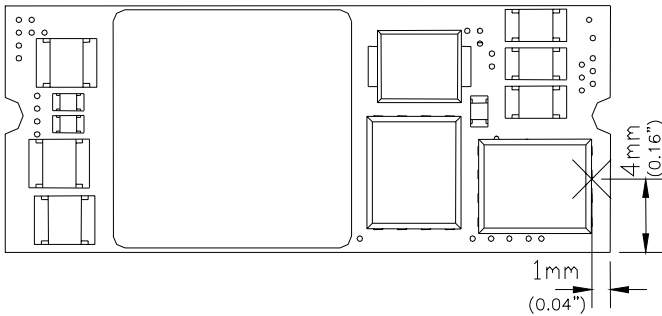
Figure 39: Temperature measurement location * The allowed maximum hot spot temperature is defined at 125 °C.
