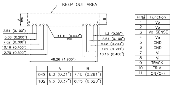
RECOMMENDED P.W.B. PAD LAYOUT
