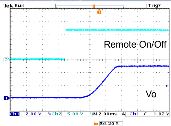
Figure 14: Turn on Using Remote On/Off with external capacitors ( C_o = 5000 \mu F ), 5.0V/16A out
