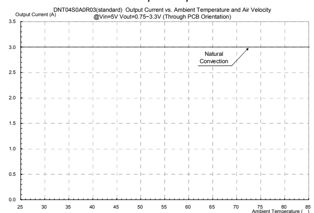
Figure 33: Output current vs. ambient temperature and air velocity @ V_{in}=5V , V_{out}=0.75V\sim 3.63V (Through PCB Orientation)
