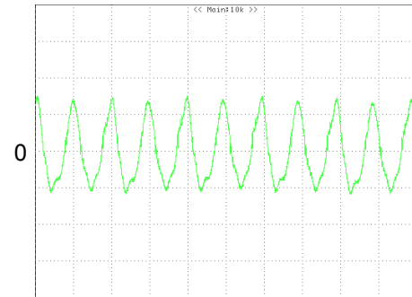
Figure 11: Input Terminal Ripple Current, i_c , at full rated output current and nominal input voltage with 12µH source impedance and 100µF electrolytic capacitor (100 mV/div, 2µs/div)
