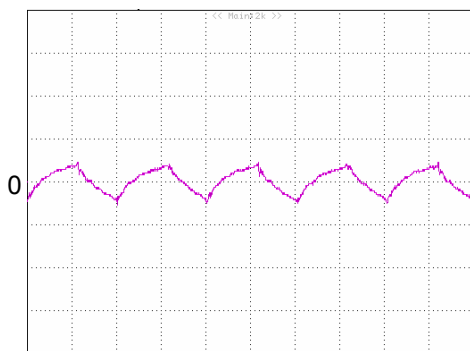
Figure 14: Output voltage ripple at nominal input voltage and rated load current ( I_o=40A ) (100 mV/div, 1µs/div) Load capacitance: 1µF ceramic capacitor and 10µF tantalum capacitor. Bandwidth: 20 MHz. Scope measurements should be made using a BNC cable (length shorter than 20 inches). Position the load between 51 mm to 76 mm (2 inches to 3 inches) from the module.
