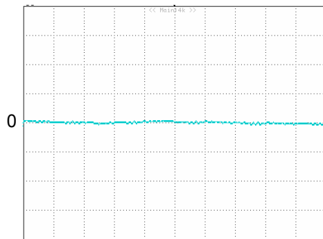
Figure 12: Input reflected ripple current, i_s , through a 12µH source inductor at nominal input voltage and rated load current (20 mV/div, 2µs/div)
