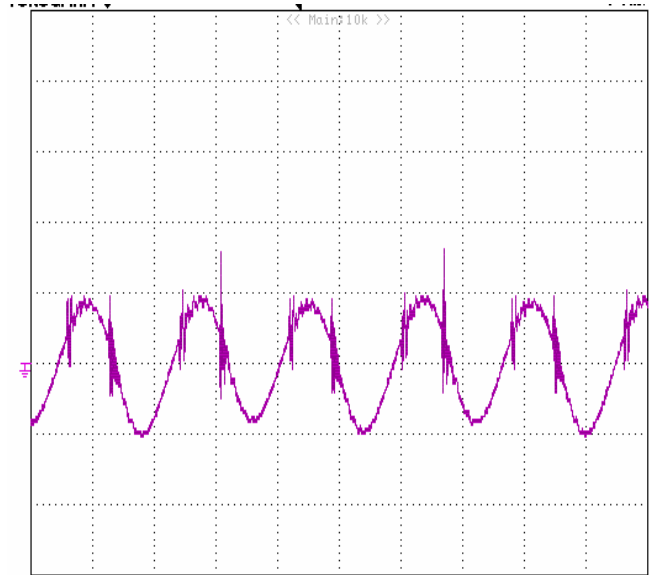
Figure 14: Output voltage ripple at nominal input voltage and rated load current (100mV/div). Load capacitance: 330uF aluminum, 1uF ceramic capacitor and 10uF Flow ESR capacitor. Bandwidth: 20 MHz. Scope measurement should be made using a BNC cable (length shorter than 20 inches). Position the load between 51 mm to 76 mm (2 inches to 3 inches) from the module.
