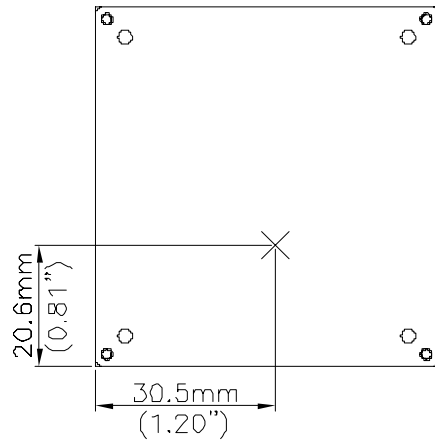
Figure 20: Temperature measurement location * The allowed maximum hot spot temperature is defined at 108 °C
