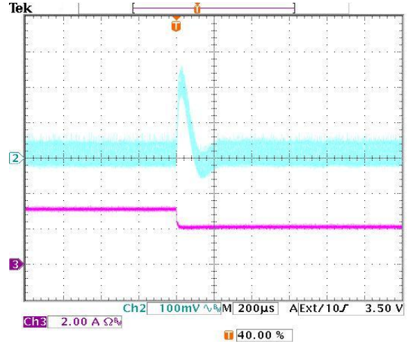
Figure 6: Output voltage response to step-change in load current (75%-50% of I_o , max; di/dt = 2.5A/\mu s ).
