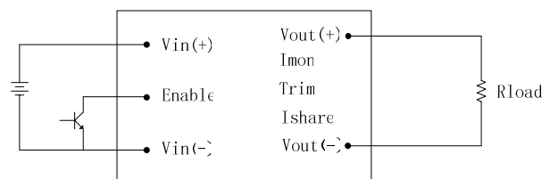
Figure 15: Remote on/off implementation
