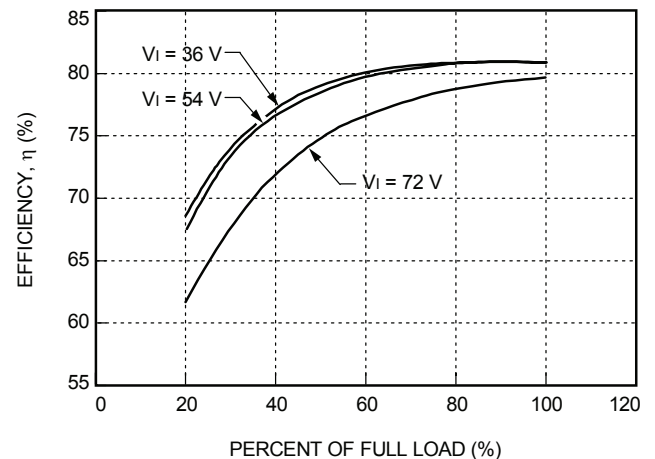
Figure 14. DW025ACL-M Typical Converter Efficiency
