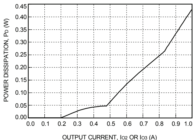
Figure 26. DW025ABK-M, Losses Associated with \pm 12 V Output, P_{s2}/P_{s3}
