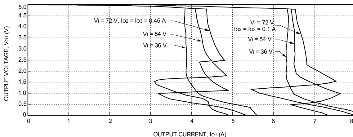
Figure 11. DW025ACL-M Typical 5 V Output Characteristics
