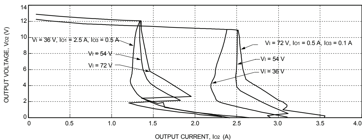
Figure 10. DW025ABK-M Typical 12 V Output Characteristics
