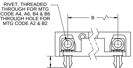
RIGHT ANGLE PLASTIC BRACKET WITH BOARD LOCK
