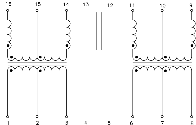
SCHEMATIC
