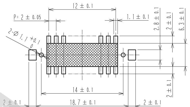
RECOMMENDED PATTEN(2:1)
