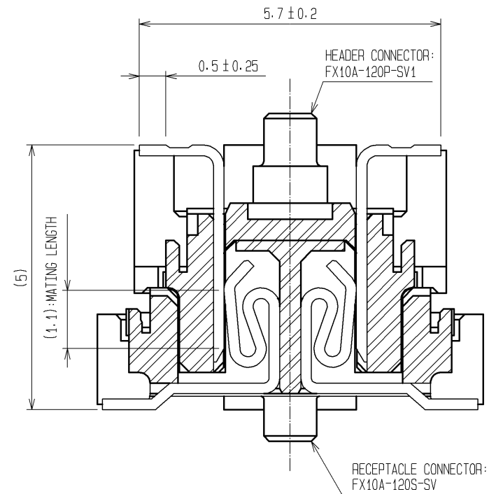
CROSS CUT SECTION (10:1)
