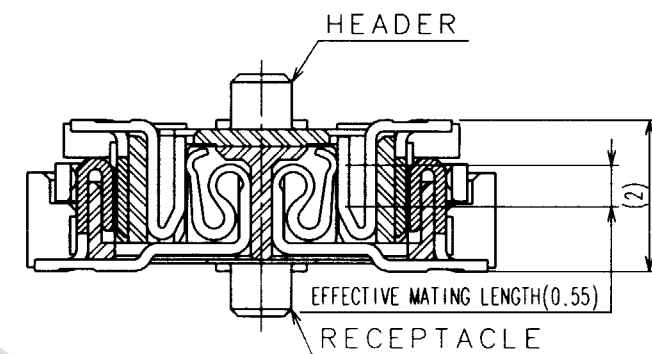
SIGNAL PORTION CROSS SECTION (10:1)
