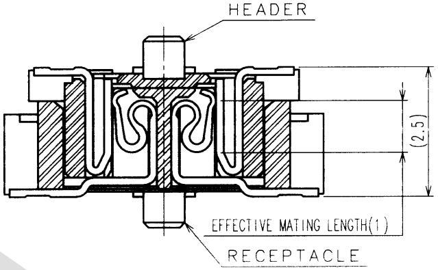
SIGNAL PORTION CROSS SECTION (10:1)
