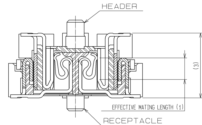
SIGNAL PORTION CROSS SECTION (10:1)
