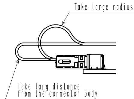
Application of cable bend back
