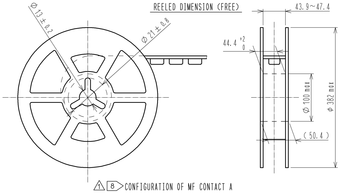
CONTACT AREA OF MF CONTACT A
