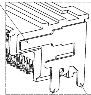
SOLDERING POLE2 OF MF CONTACT A
