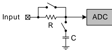
Figure 25.4. ADC RC Input Filter Configuration
