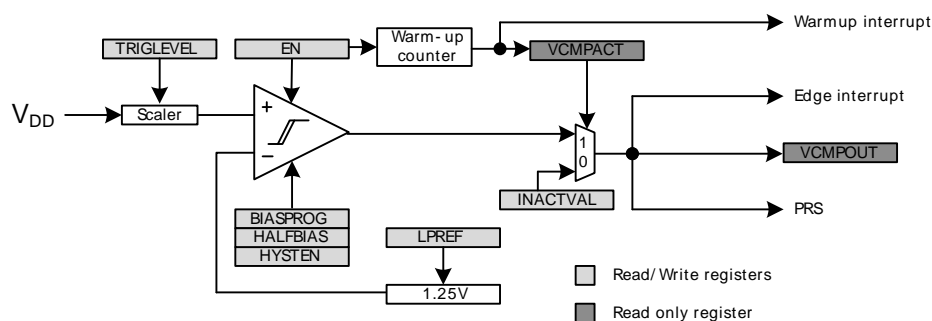
Figure 24.1. VCMP Overview
