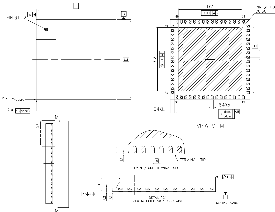
Figure 4.2. QFN64
