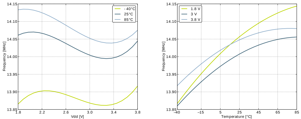
Figure 3.10. Calibrated HFRCO 21 MHz Band Frequency vs Supply Voltage and Temperature
