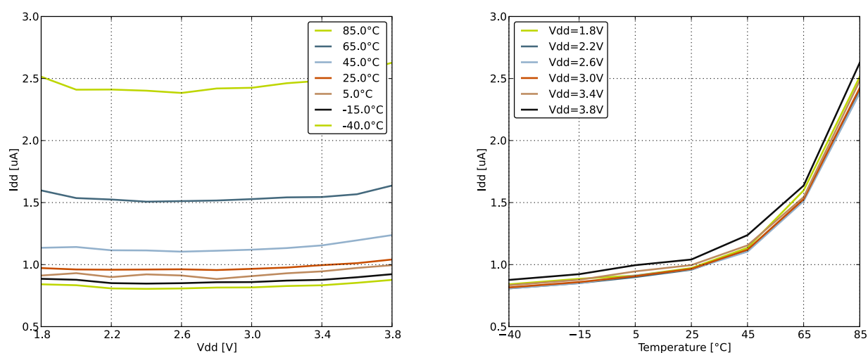
Figure 3.2. EM3 current consumption.
