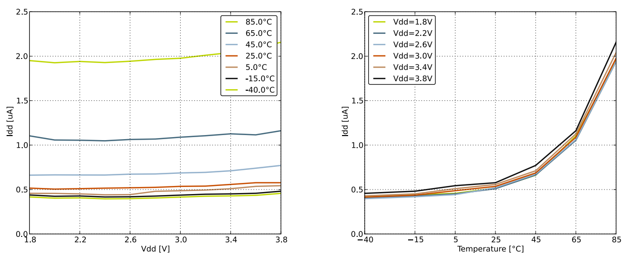
Figure 3.3. EM4 current consumption.
