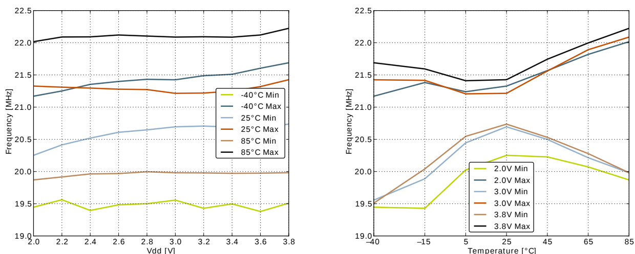
Figure 3.16. Calibrated HFRCO 28 MHz Band Frequency vs Supply Voltage and Temperature
