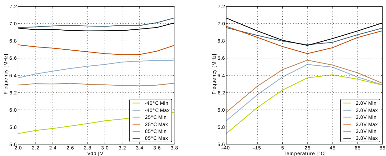
Figure 3.13. Calibrated HFRCO 11 MHz Band Frequency vs Supply Voltage and Temperature
