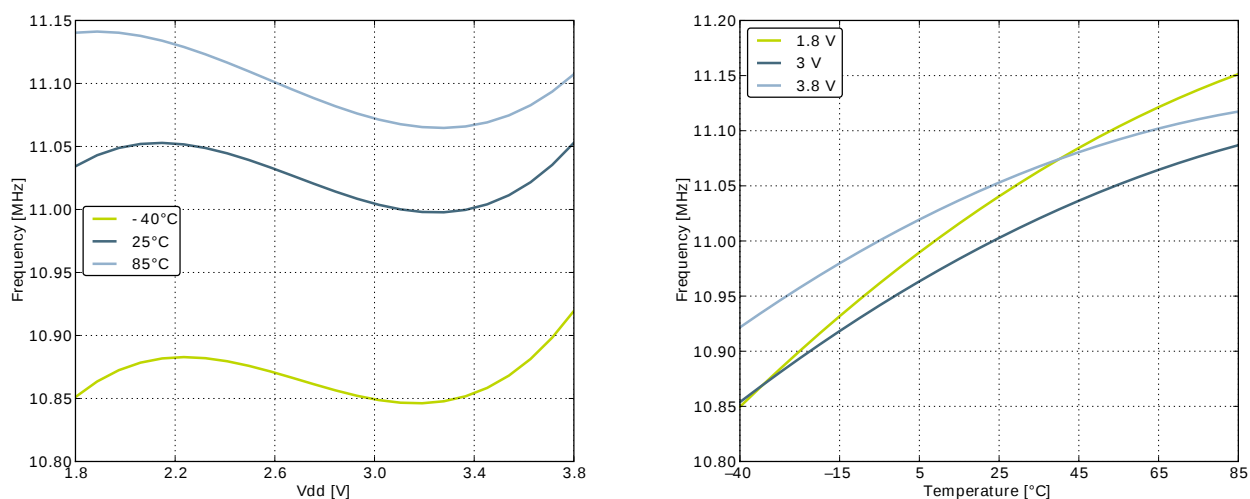
Figure 3.12. Calibrated HFRCO 14 MHz Band Frequency vs Supply Voltage and Temperature
