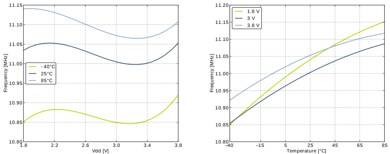
Figure 3.19. Calibrated HFRCO 14 MHz Band Frequency vs Supply Voltage and Temperature
