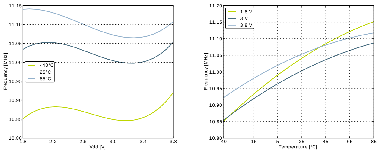
Figure 3.19. Calibrated HFRCO 14 MHz Band Frequency vs Supply Voltage and Temperature
