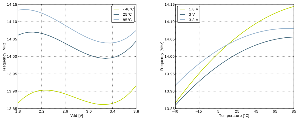
Figure 3.20. Calibrated HFRCO 21 MHz Band Frequency vs Supply Voltage and Temperature
